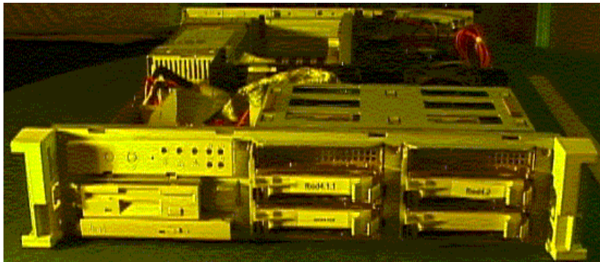
Fig 2: Screamer II - 2I2U, 4xSCA-2 hot-swap, RAID 0, 1, 5, Ultra 160/320
