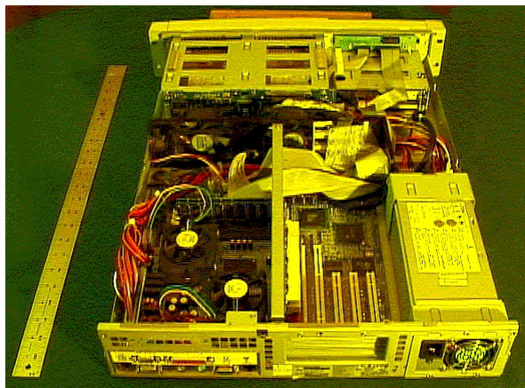
Fig 3: Screamer II 2I2U. Rear view.
